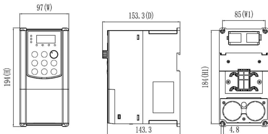
4T 4.0G—5.5G structure diagram and dimension
