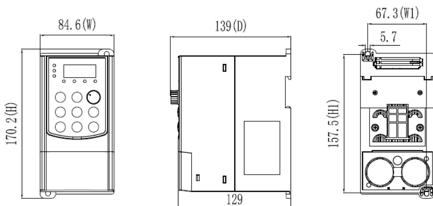
2S 2.2G & 4T—2.2G structure diagram and dimension
