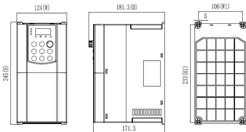
2T 7.5G-11G & 2S 4.0G—5.5G structure diagram and dimension
