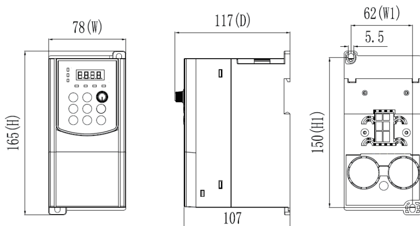
2S 0.7G—1.5G structure diagram and dimension
