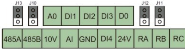
Control circuit terminal
